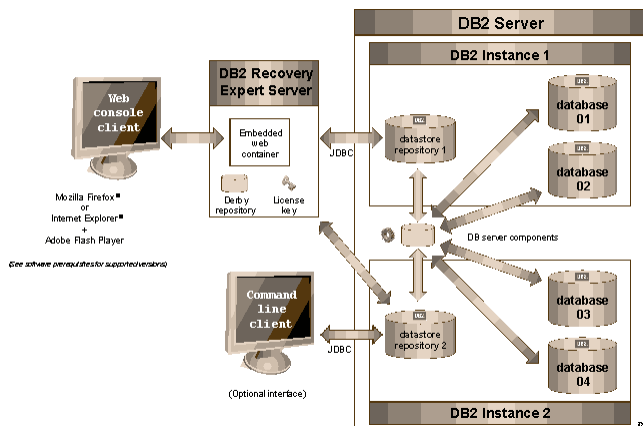
Figure 1. Db2 Recovery Expert architecture diagram
